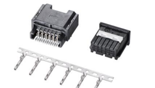
JJL2011HC系列 2.0mm间距 双锁车规级WTB单排插头 Spec: JL2011HC Series 2.0mm Double Lock Gauge WTB Single Row Plug Installation type:SMT
