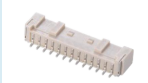
JL2019Z系列 2.0mm间距 双锁车规级WTB单排卧贴针座 Spec: JL2019Z Series 2.0mm Double Lock Gauge WTB Single Row Right Angle SMT Installation type:SMT, Right Angle
