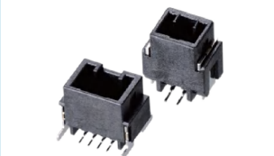
JL2024M系列 2.0mm间距 双锁车规级WTB单双排立贴针座 Spec: JL2024M Series 2.0mm Double Lock Gauge WTB Single Double Row Right Angle SMT Installation type:SMT, Through-hole
