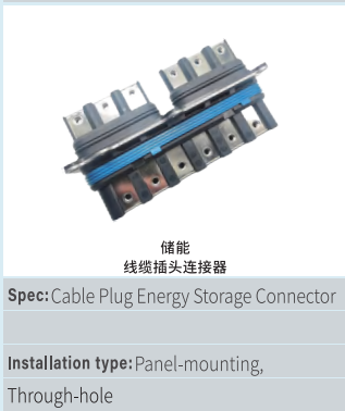
小型电源 90°公头连接器 Spec: Small Power Supply 90° Degree Male Connector Installation type: Through-hole, Right Angle
