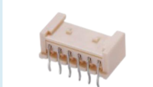
JL2514R系列 2.5mm间距 双锁车规级WTB单排90°针座 Spec: JL2514R Series 2.5mm Double Lock Gauge WTB Single Row Right Angle Installation type:Through-hole, Right Angle
