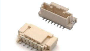
2.0mm间距 WTB针座连接器 Spec:2.0mm WTB SMT Wafer Connector Installation type:SMT, Right Angle
