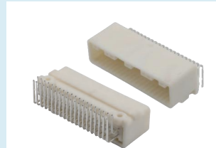
2.2mm间距 BMS信号连接器弯公-白色 Spec:2.2mm BMS Right Angle Male Signal Connector White Installation type:Through-hole, Right Angle
