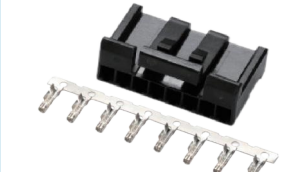
JL2020H系列 2.0mm间距 双锁车规级WTB单排插头 Spec: JL2020H Series 2.0mm Double Lock Gauge WTB Single Row Plug Installation type:Free-hanging
